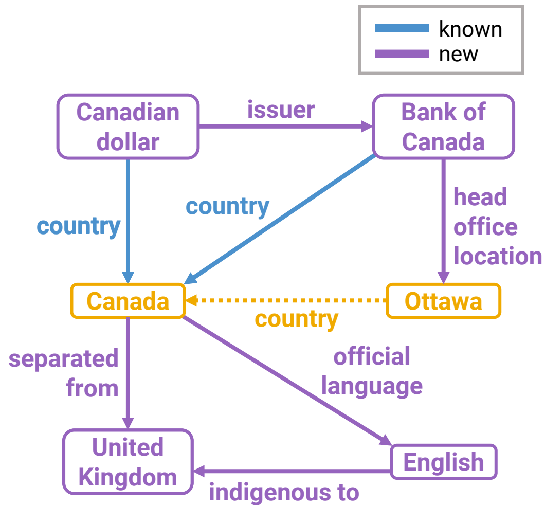
Inference Graph
