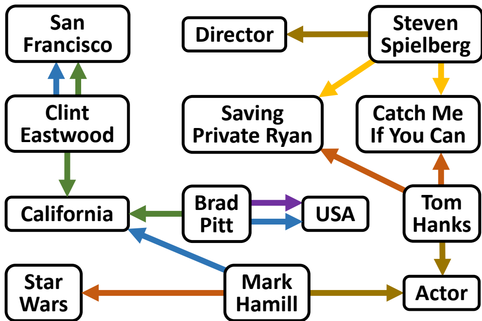
Knowledge Graph
