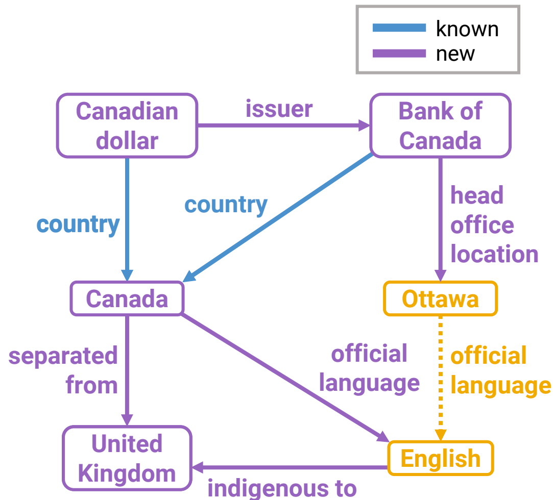
Inference Graph
